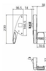
PUSH PAD SYSTÉM
