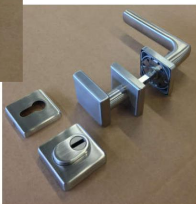
set DKHR s klikou Dallas a rozetami HR15P + HR9
